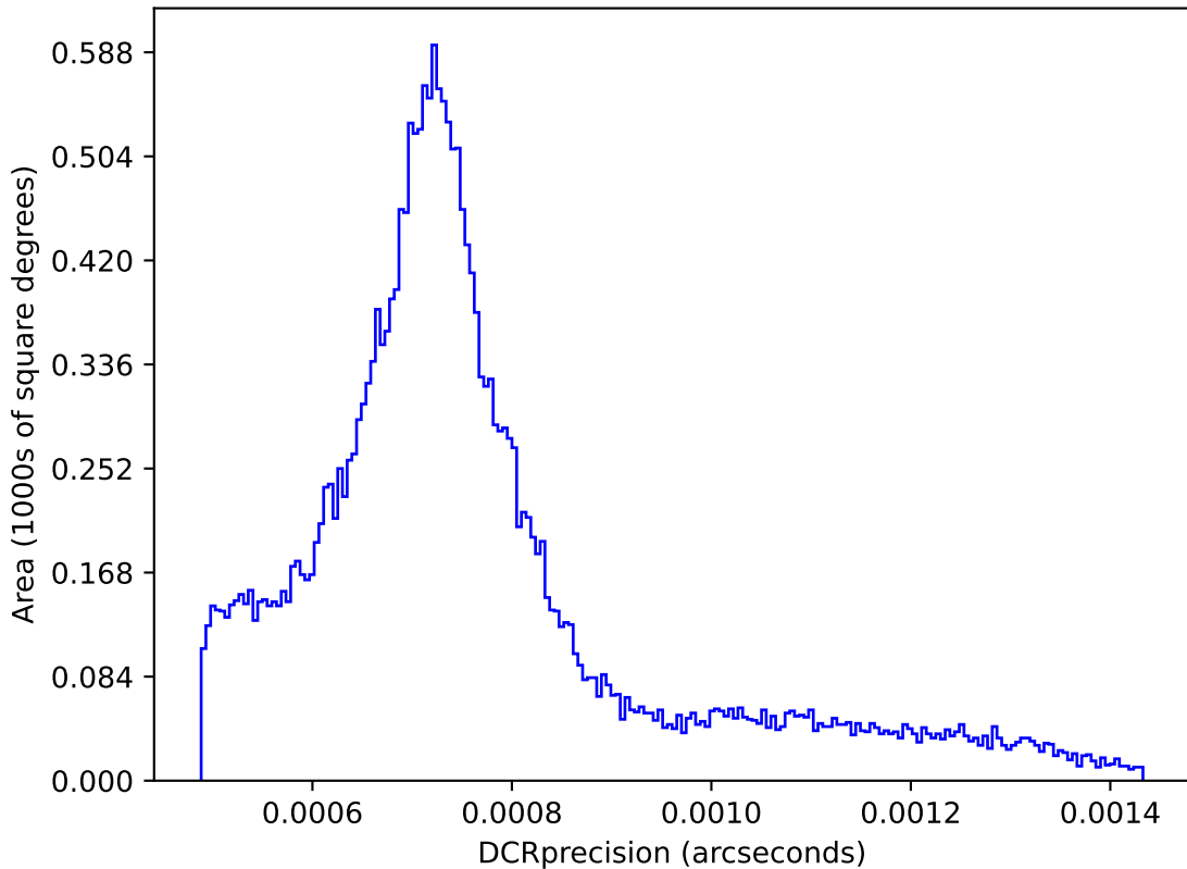
too_elab_r8_d3_gz_v3.4_10yrs : DCRprecision
