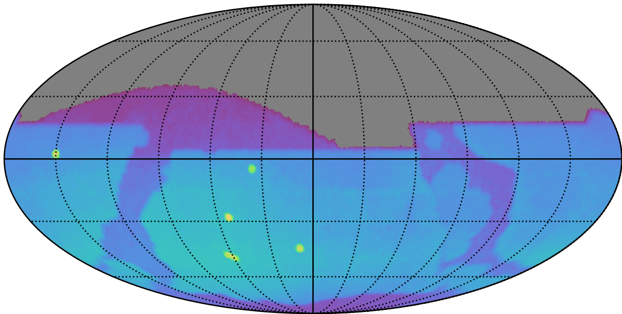
too_elab_r8_d3_gz_v3.4_10yrs : Brown Dwarf, L7
