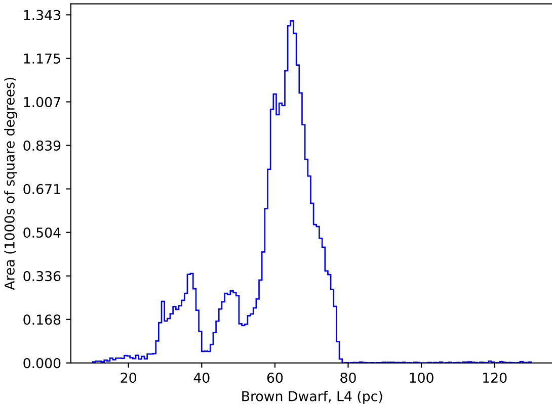
too_elab_r8_d3_gz_v3.4_10yrs : Brown Dwarf, L4
