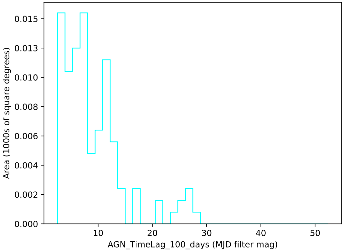
too_elab_r8_d3_gz_v3.4_10yrs u band: AGN_TimeLag_100_days
