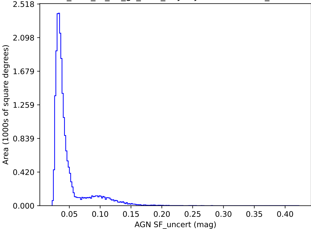
too_elab_r8_d3_gz_v3.4_10yrs y band: AGN SF_uncert
