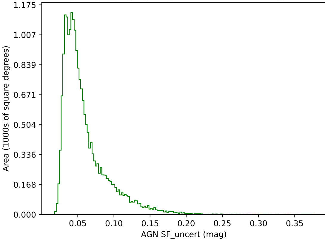
too_elab_r8_d3_gz_v3.4_10yrs g band: AGN SF_uncert
