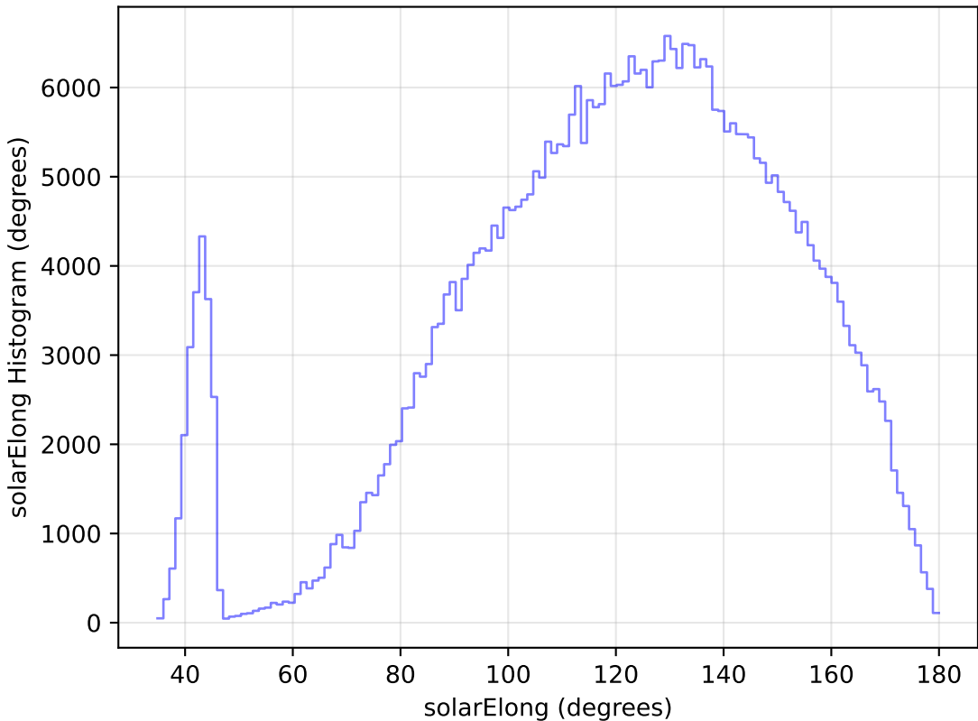
too_elab_r8_d3_gz_v3.4_10yrs WFD z band: solarElong Histogram
