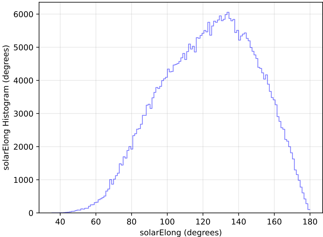
too_elab_r8_d3_gz_v3.4_10yrs WFD y band: solarElong Histogram
