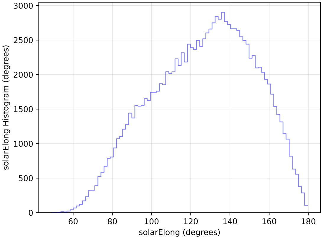
too_elab_r8_d3_gz_v3.4_10yrs WFD u band: solarElong Histogram
