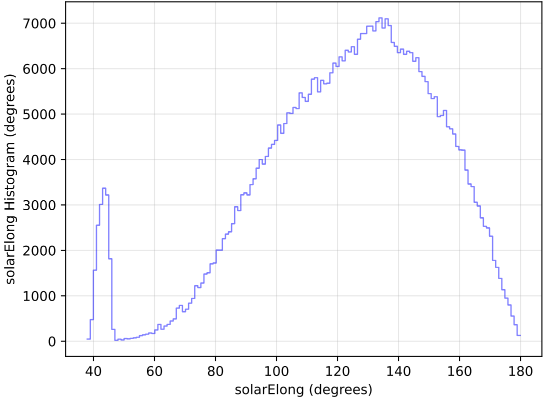
too_elab_r8_d3_gz_v3.4_10yrs WFD r band: solarElong Histogram
