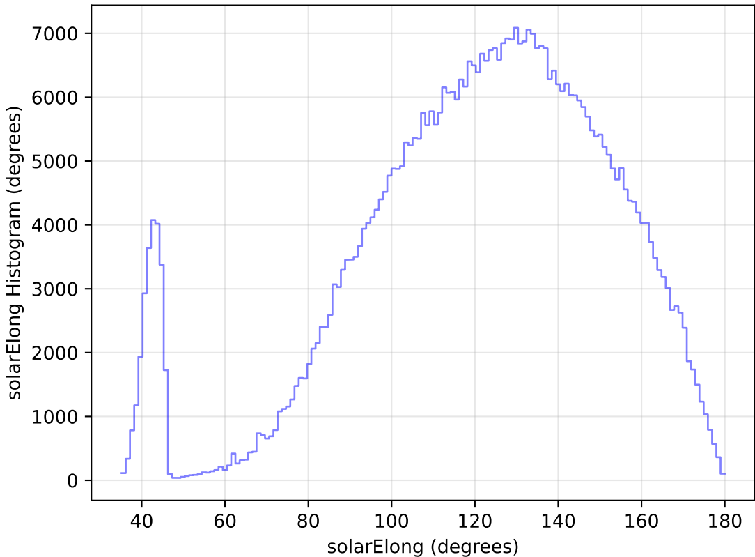
too_elab_r8_d3_gz_v3.4_10yrs WFD i band: solarElong Histogram
