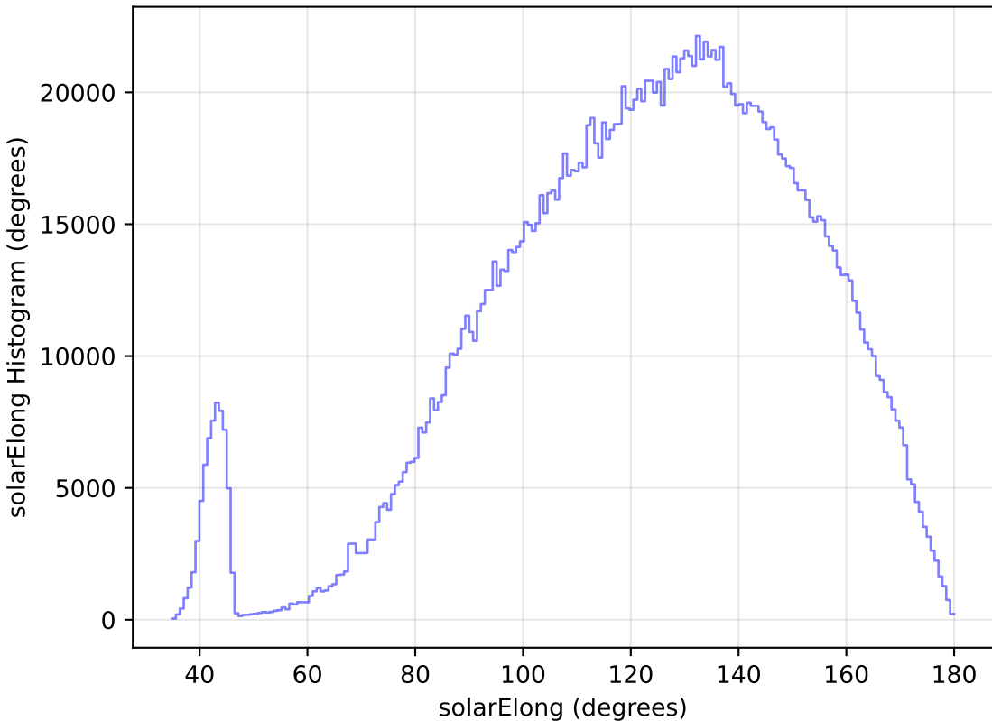
too_elab_r8_d3_gz_v3.4_10yrs WFD all bands: solarElong Histogram
