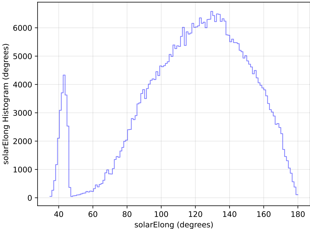
too_elab_r8_d3_gz_v3.4_10yrs All sky z band: solarElong Histogram
