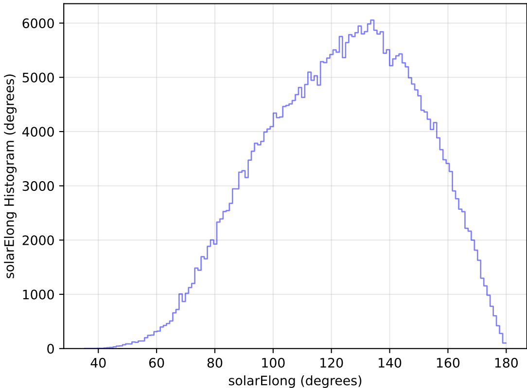
too_elab_r8_d3_gz_v3.4_10yrs All sky y band: solarElong Histogram
