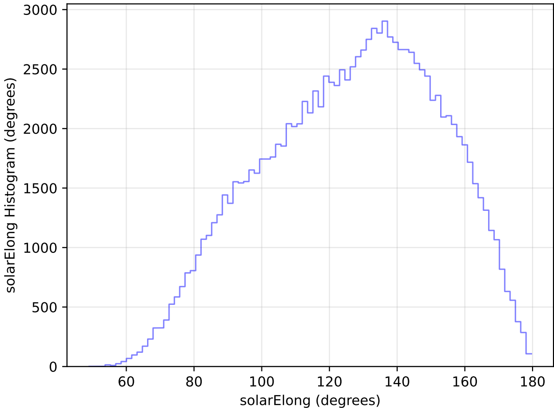
too_elab_r8_d3_gz_v3.4_10yrs All sky u band: solarElong Histogram
