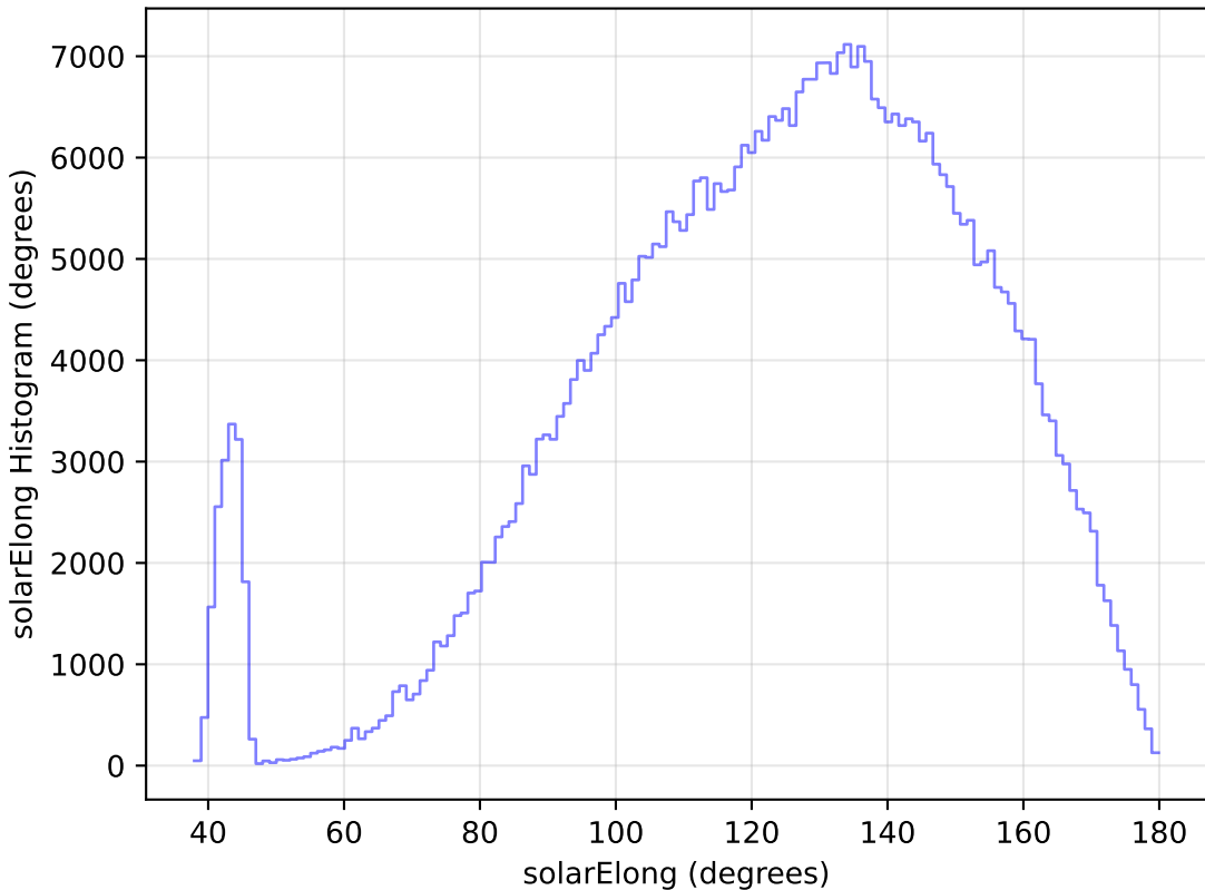
too_elab_r8_d3_gz_v3.4_10yrs All sky r band: solarElong Histogram
