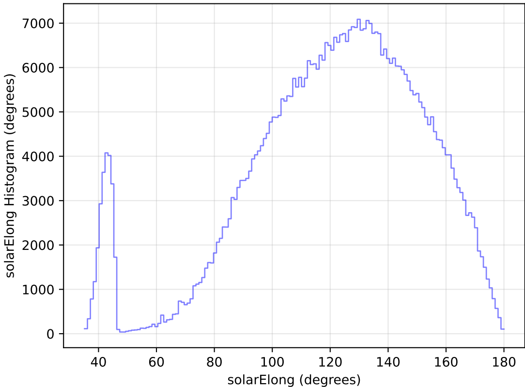
too_elab_r8_d3_gz_v3.4_10yrs All sky i band: solarElong Histogram
