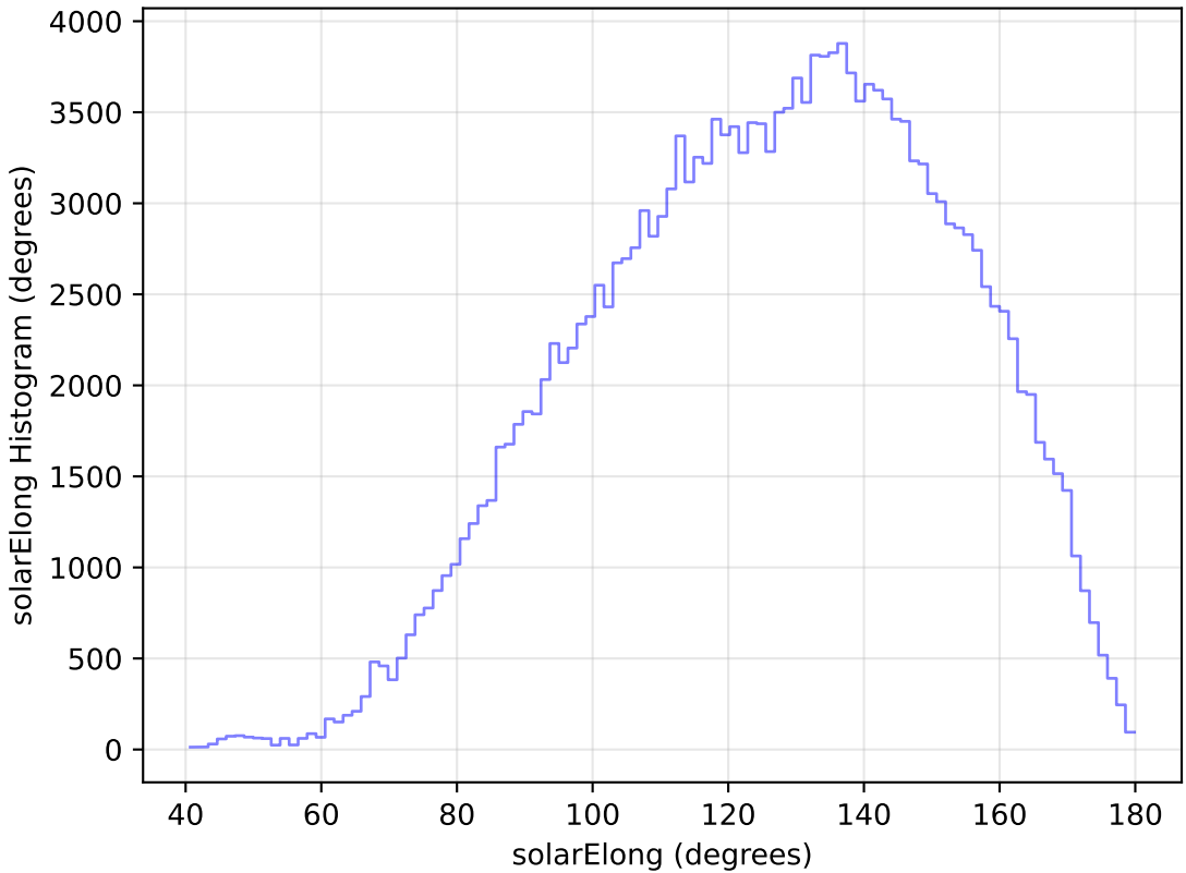
too_elab_r8_d3_gz_v3.4_10yrs All sky g band: solarElong Histogram
