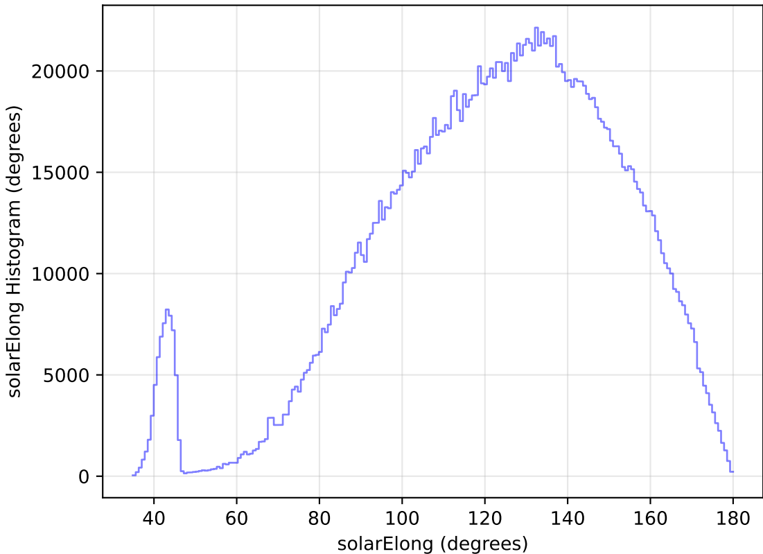
too_elab_r8_d3_gz_v3.4_10yrs All sky all bands: solarElong Histogram
