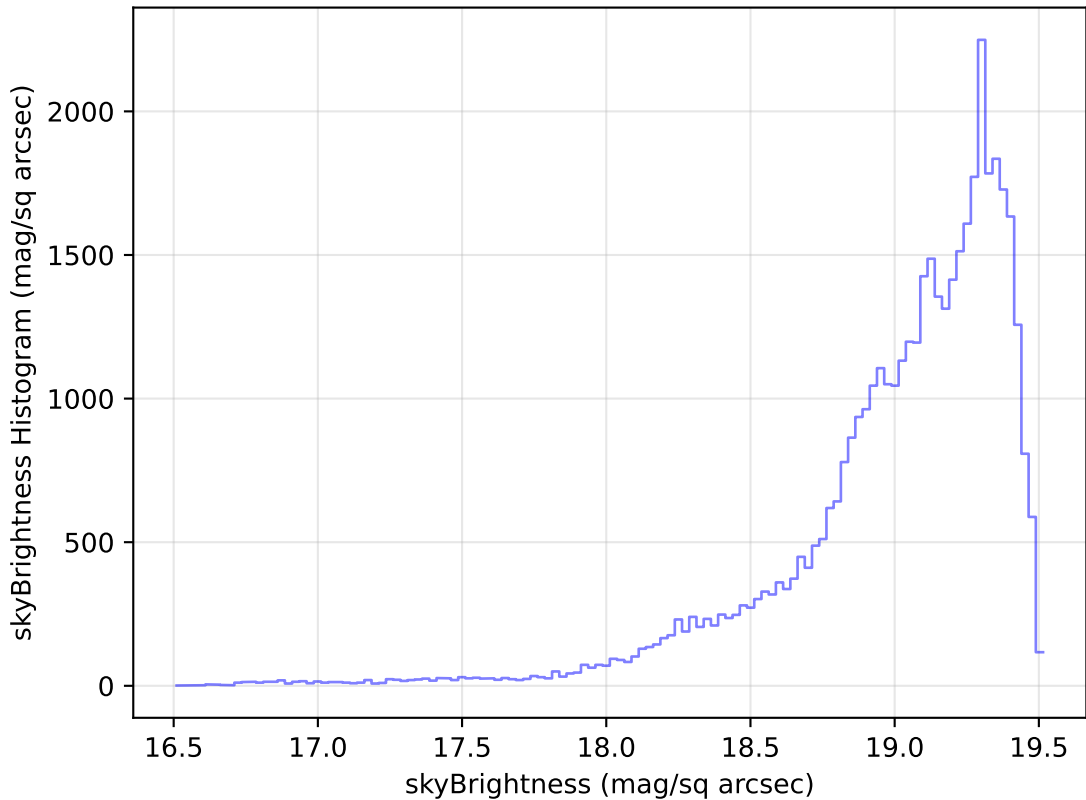
too_elab_r8_d3_gz_v3.4_10yrs Yr 1 z band: skyBrightness Histogram
