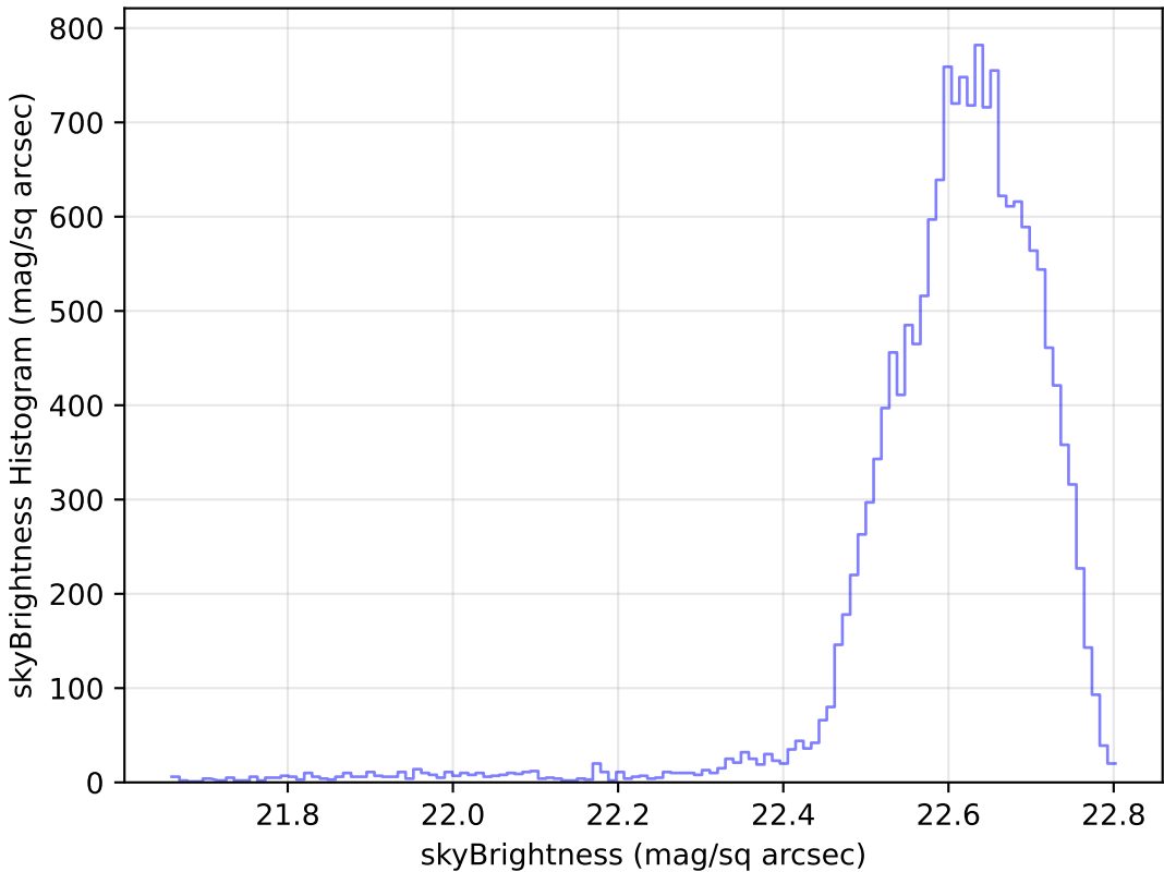
too_elab_r8_d3_gz_v3.4_10yrs Yr 1 u band: skyBrightness Histogram
