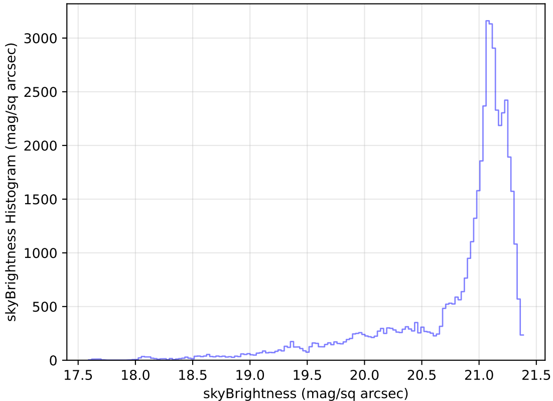
too_elab_r8_d3_gz_v3.4_10yrs Yr 1 r band: skyBrightness Histogram
