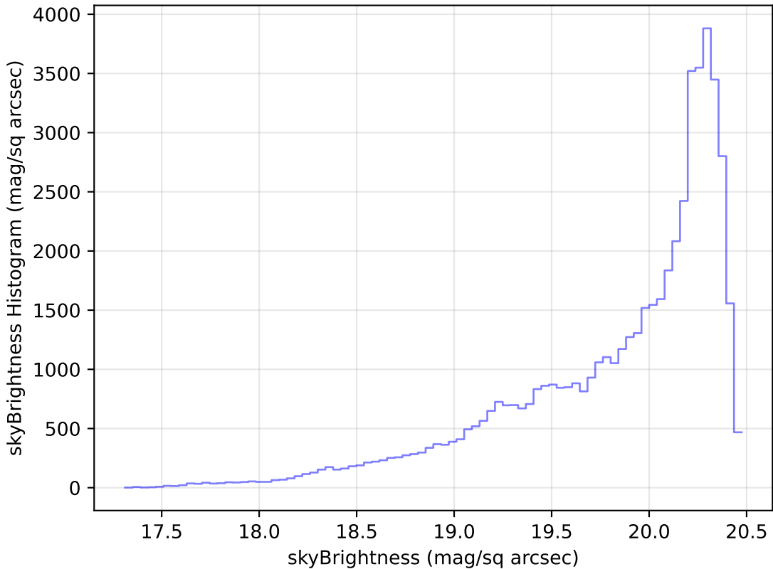
too_elab_r8_d3_gz_v3.4_10yrs Yr 1 i band: skyBrightness Histogram
