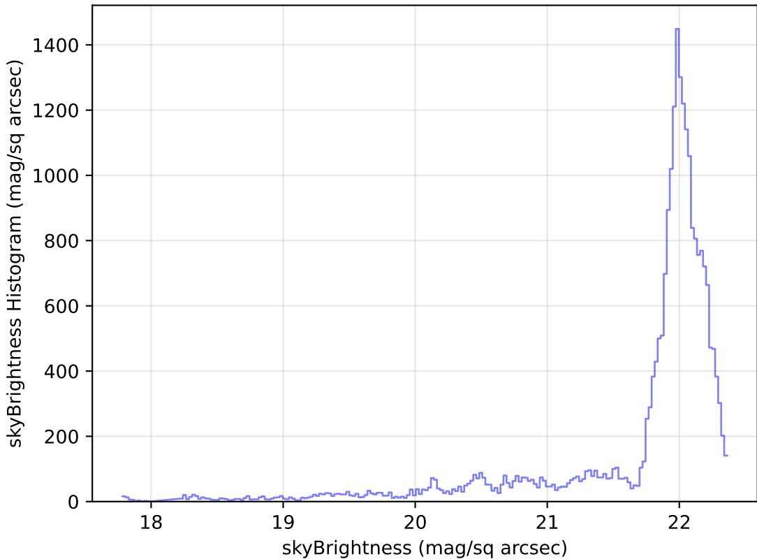
too_elab_r8_d3_gz_v3.4_10yrs Yr 1 g band: skyBrightness Histogram
