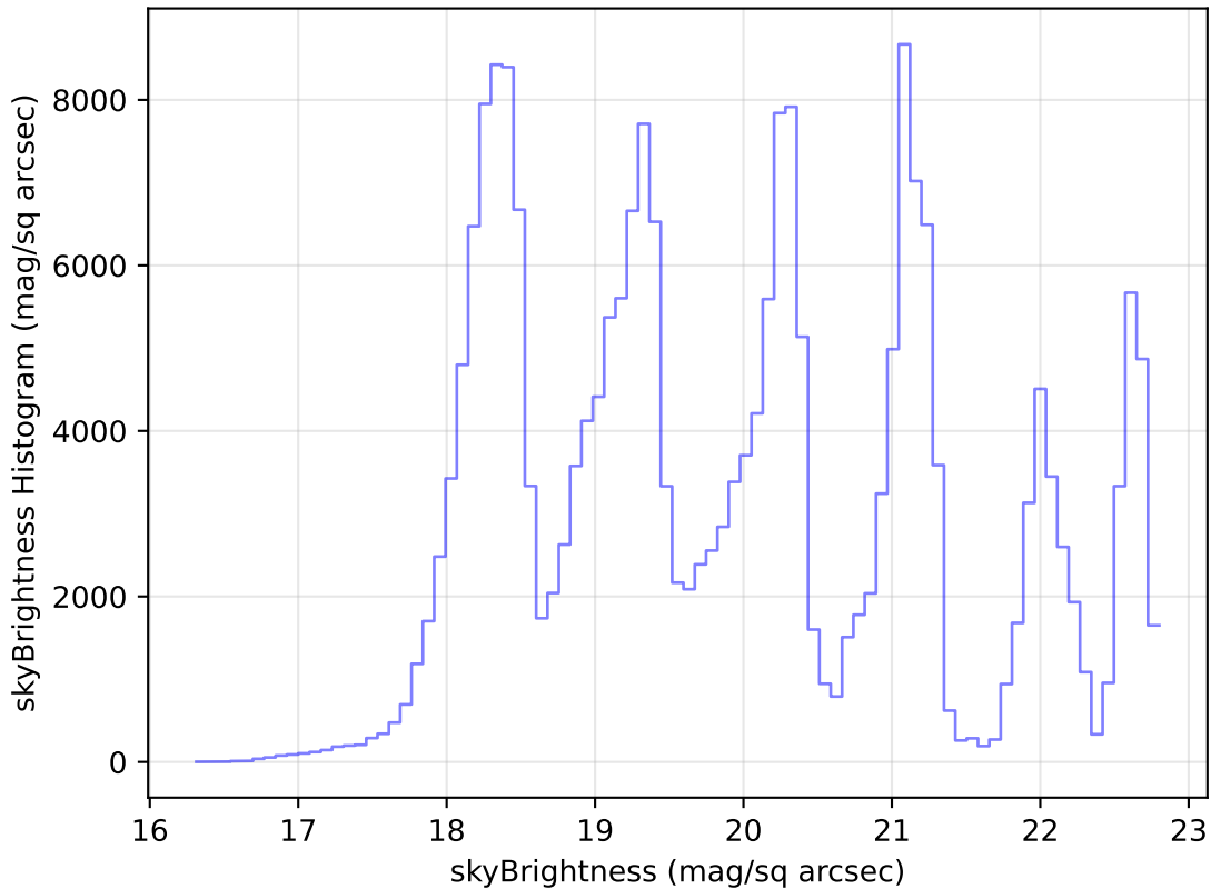
too_elab_r8_d3_gz_v3.4_10yrs Yr 1 all bands: skyBrightness Histogram
