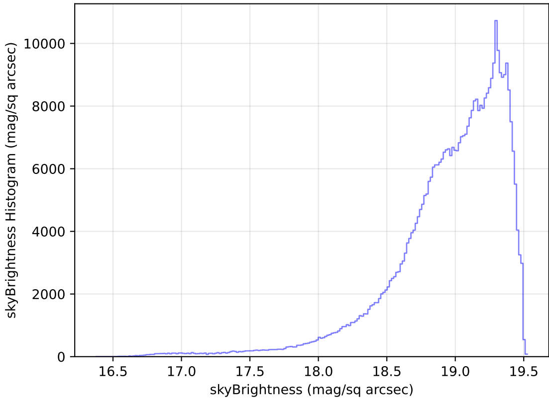
too_elab_r8_d3_gz_v3.4_10yrs WFD z band: skyBrightness Histogram
