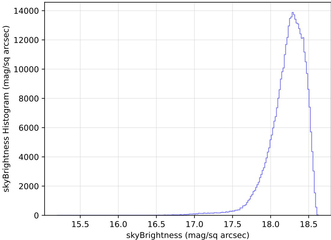
too_elab_r8_d3_gz_v3.4_10yrs WFD y band: skyBrightness Histogram
