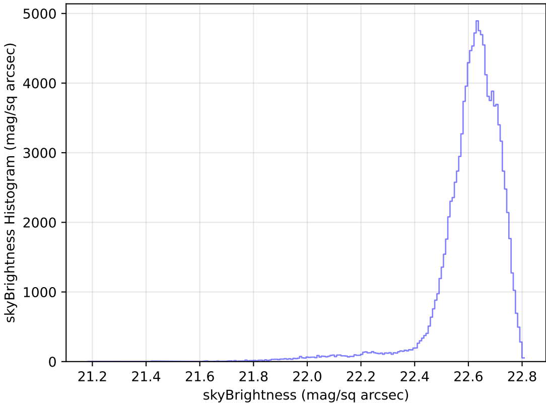
too_elab_r8_d3_gz_v3.4_10yrs WFD u band: skyBrightness Histogram
