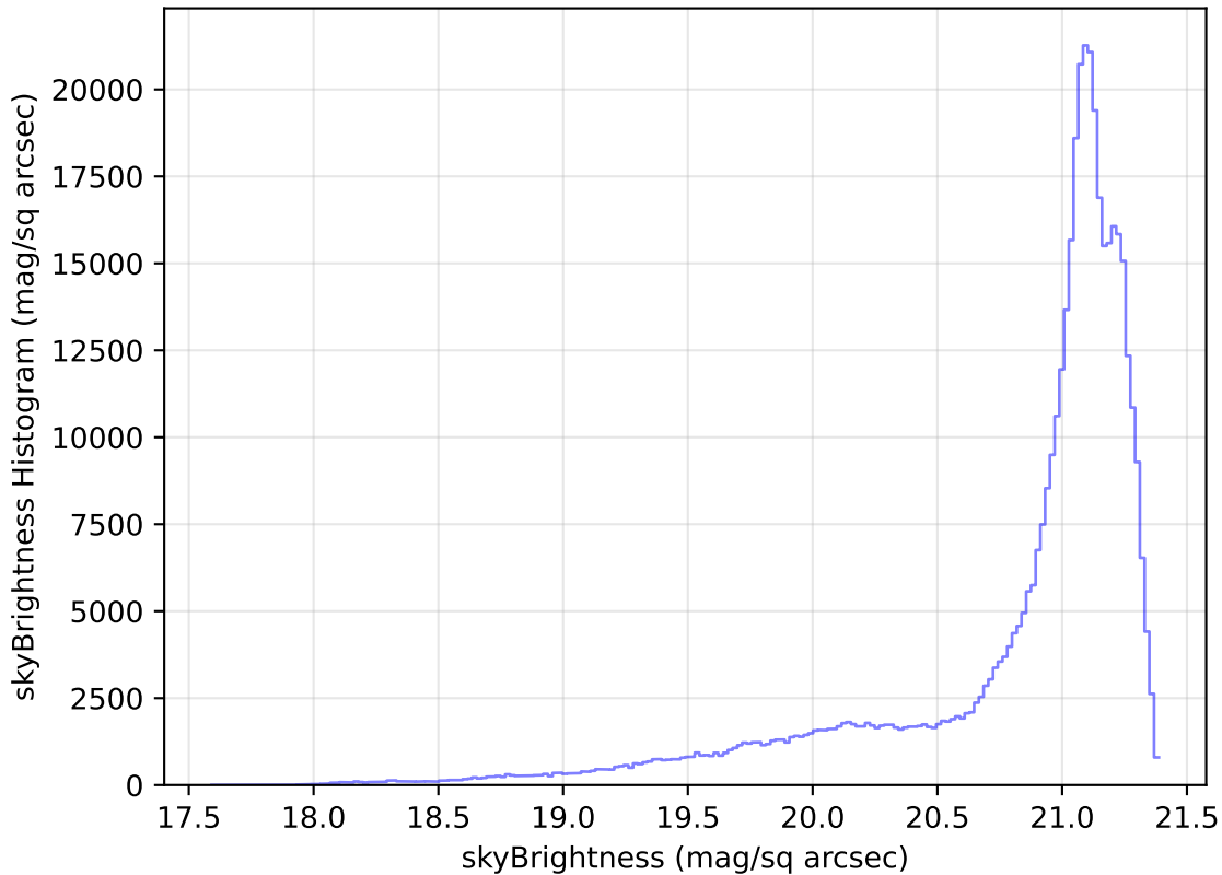
too_elab_r8_d3_gz_v3.4_10yrs WFD r band: skyBrightness Histogram
