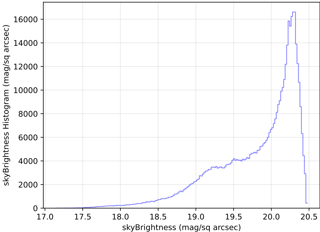
too_elab_r8_d3_gz_v3.4_10yrs WFD i band: skyBrightness Histogram
