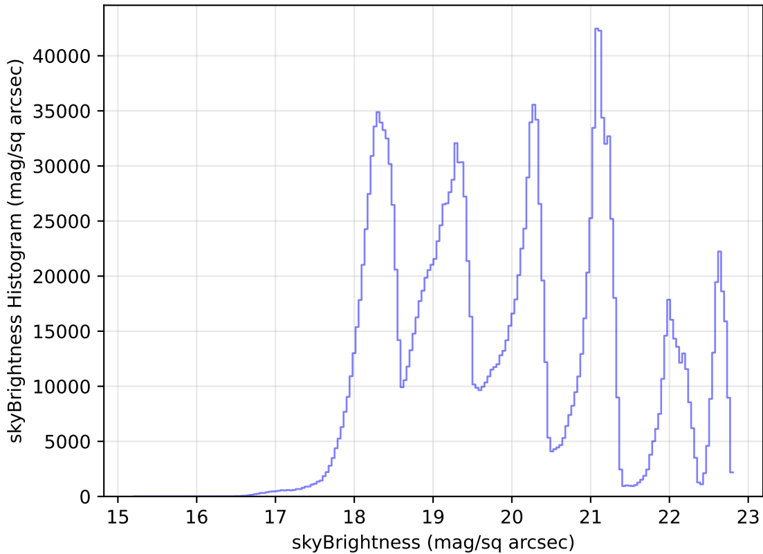
too_elab_r8_d3_gz_v3.4_10yrs WFD all bands: skyBrightness Histogram
