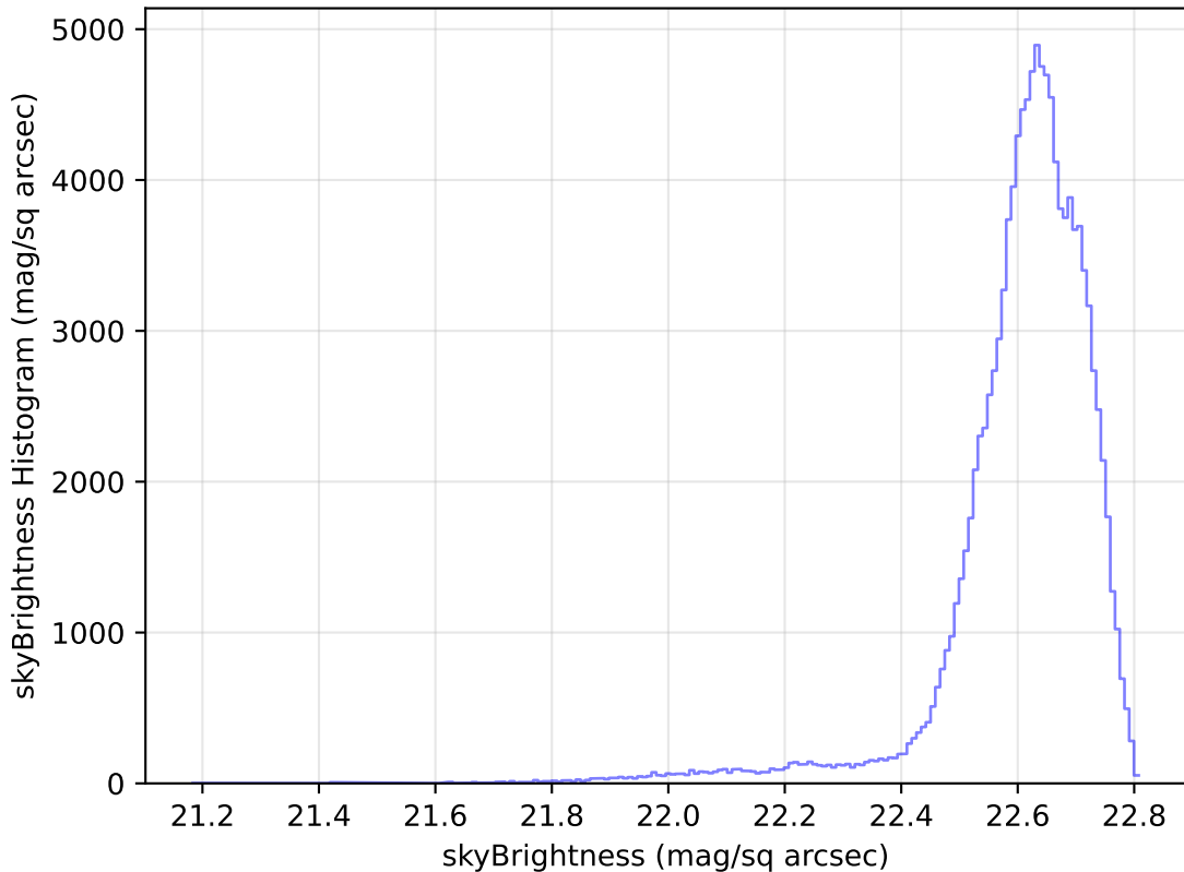
too_elab_r8_d3_gz_v3.4_10yrs All sky u band: skyBrightness Histogram
