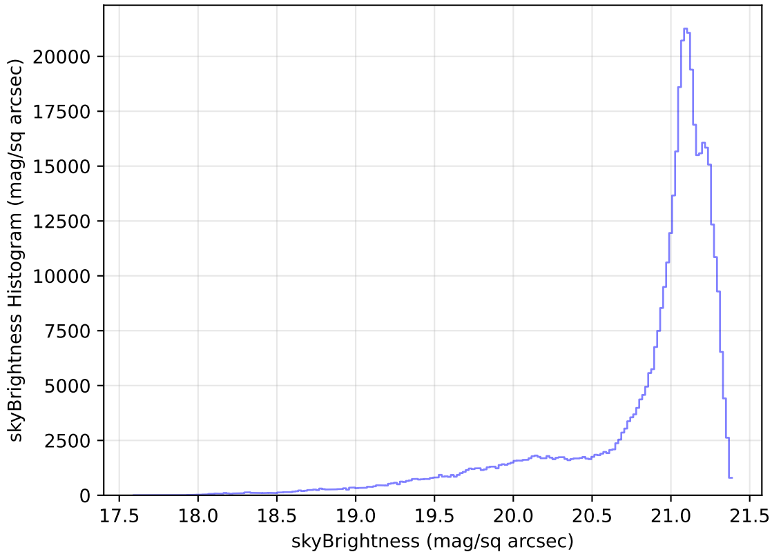
too_elab_r8_d3_gz_v3.4_10yrs All sky r band: skyBrightness Histogram
