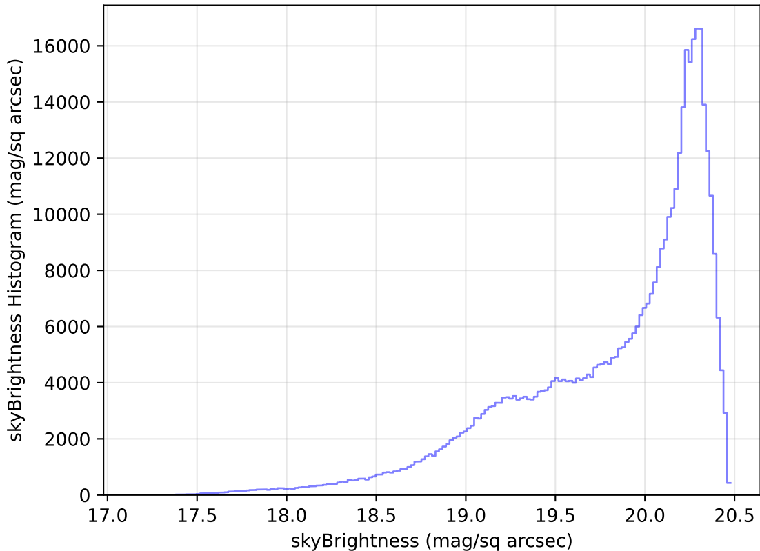
too_elab_r8_d3_gz_v3.4_10yrs All sky i band: skyBrightness Histogram
