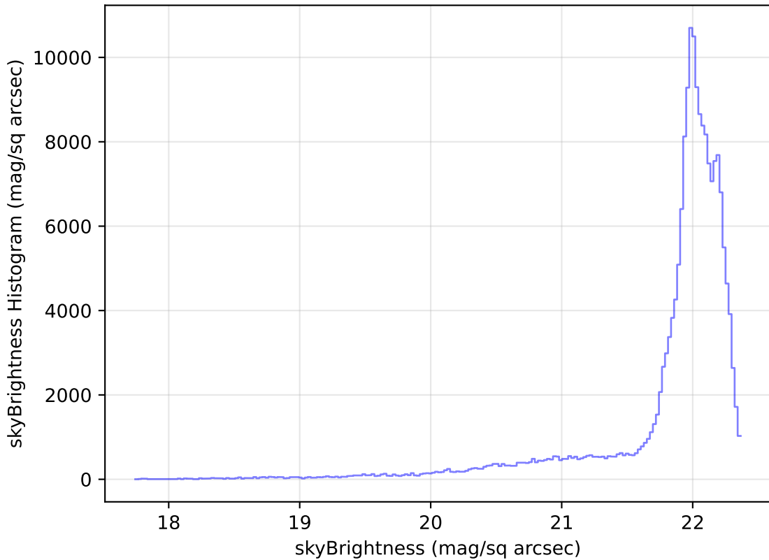
too_elab_r8_d3_gz_v3.4_10yrs All sky g band: skyBrightness Histogram
