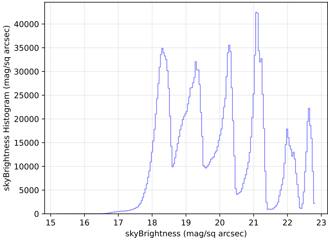
too_elab_r8_d3_gz_v3.4_10yrs All sky all bands: skyBrightness Histogram
