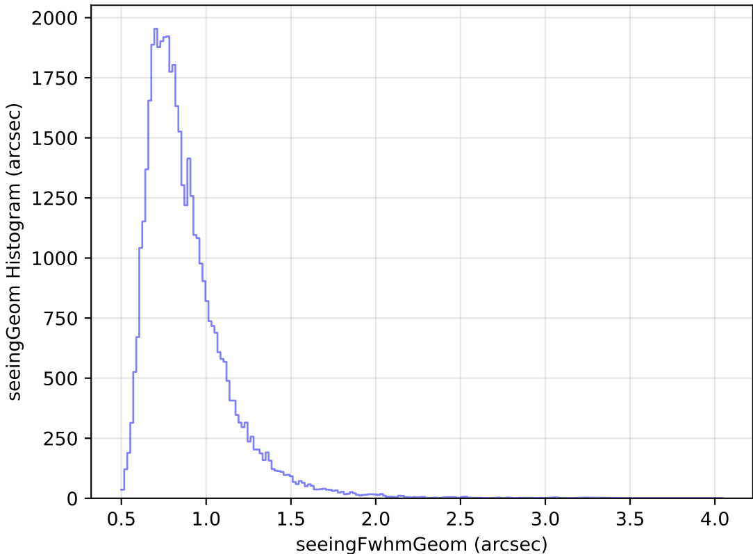
too_elab_r8_d3_gz_v3.4_10yrs Yr 1 z band: seeingGeom Histogram
