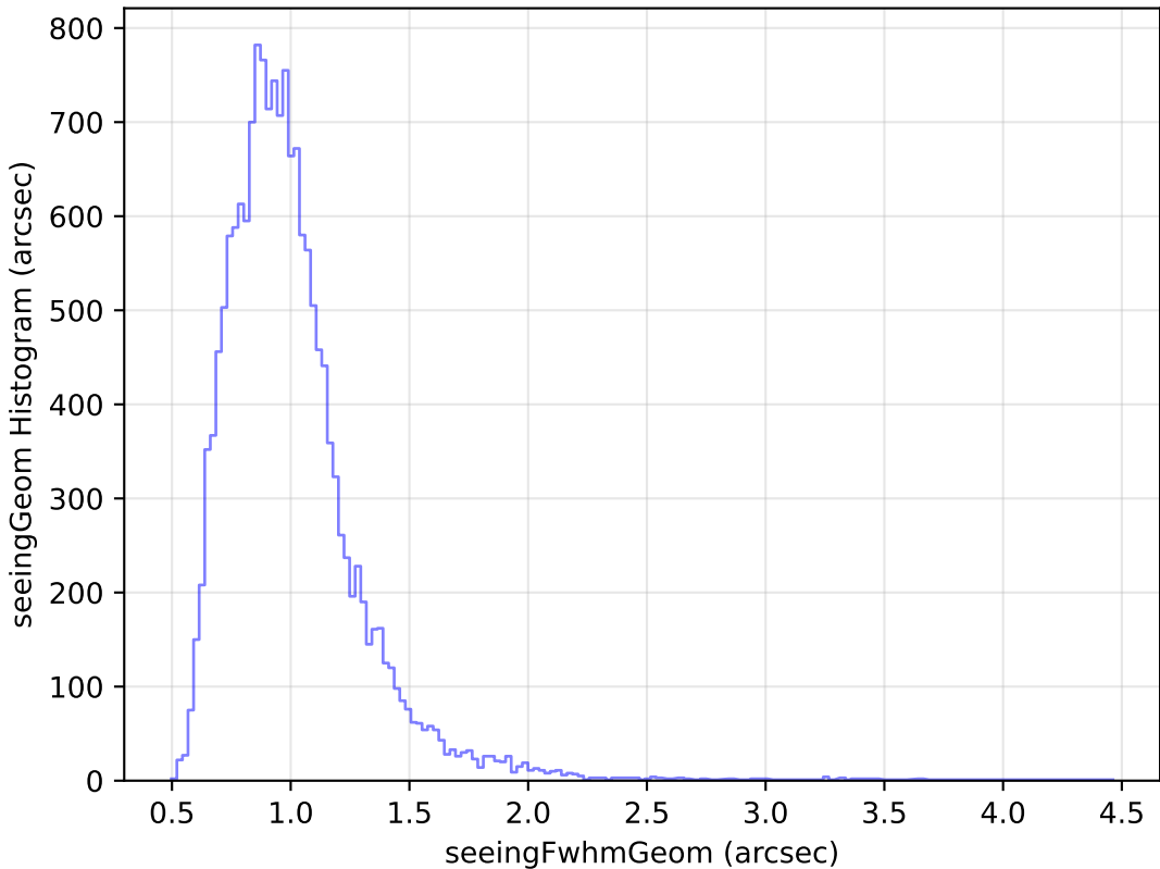
too_elab_r8_d3_gz_v3.4_10yrs Yr 1 u band: seeingGeom Histogram
