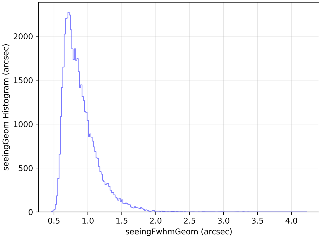
too_elab_r8_d3_gz_v3.4_10yrs Yr 1 r band: seeingGeom Histogram
