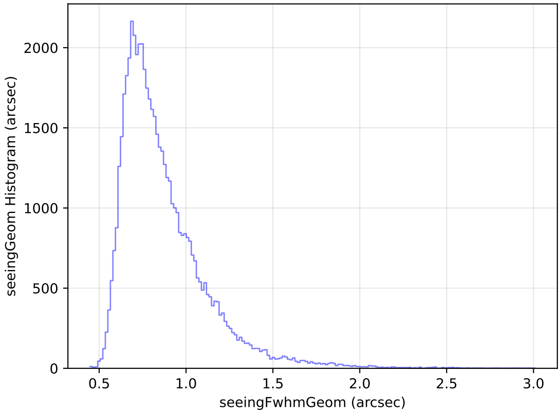
too_elab_r8_d3_gz_v3.4_10yrs Yr 1 i band: seeingGeom Histogram
