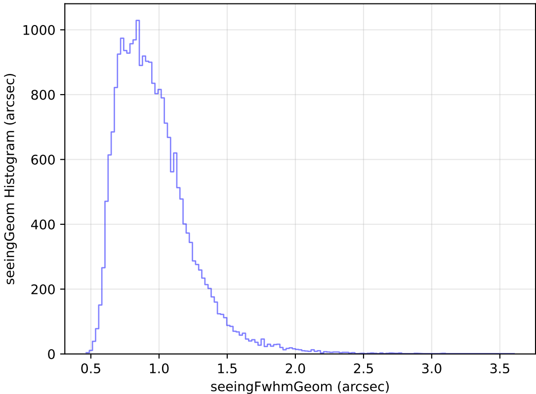
too_elab_r8_d3_gz_v3.4_10yrs Yr 1 g band: seeingGeom Histogram
