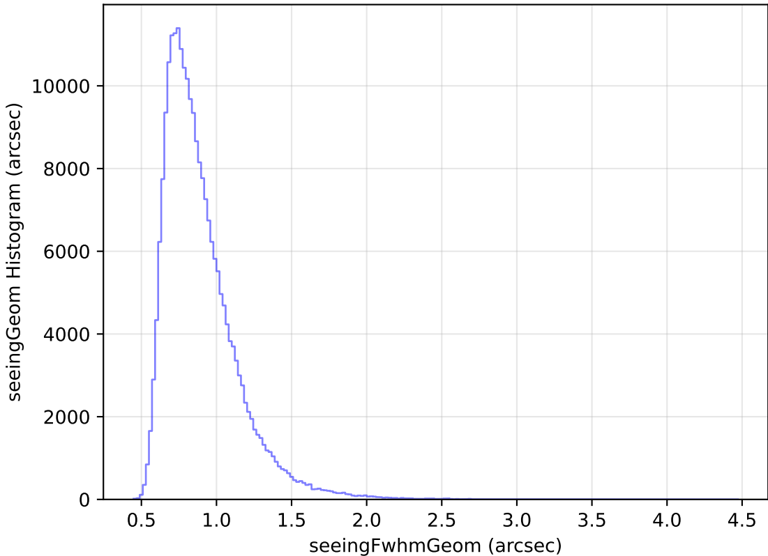
too_elab_r8_d3_gz_v3.4_10yrs Yr 1 all bands: seeingGeom Histogram
