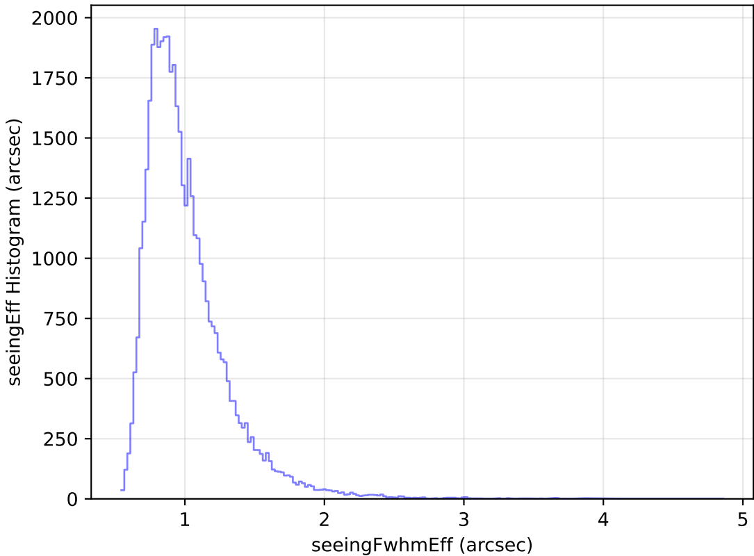
too_elab_r8_d3_gz_v3.4_10yrs Yr 1 z band: seeingEff Histogram
