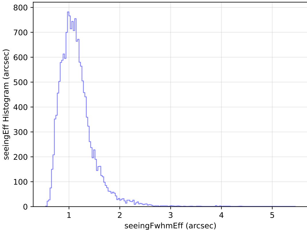
too_elab_r8_d3_gz_v3.4_10yrs Yr 1 u band: seeingEff Histogram
