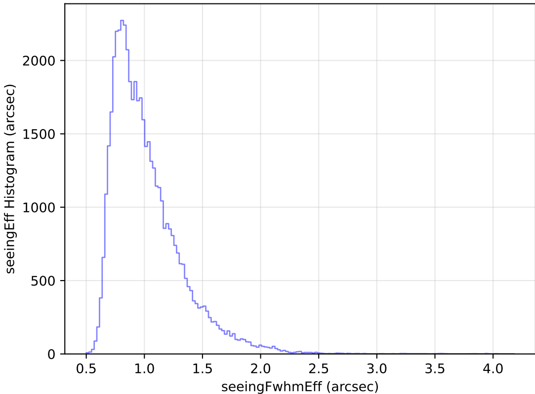
too_elab_r8_d3_gz_v3.4_10yrs Yr 1 r band: seeingEff Histogram
