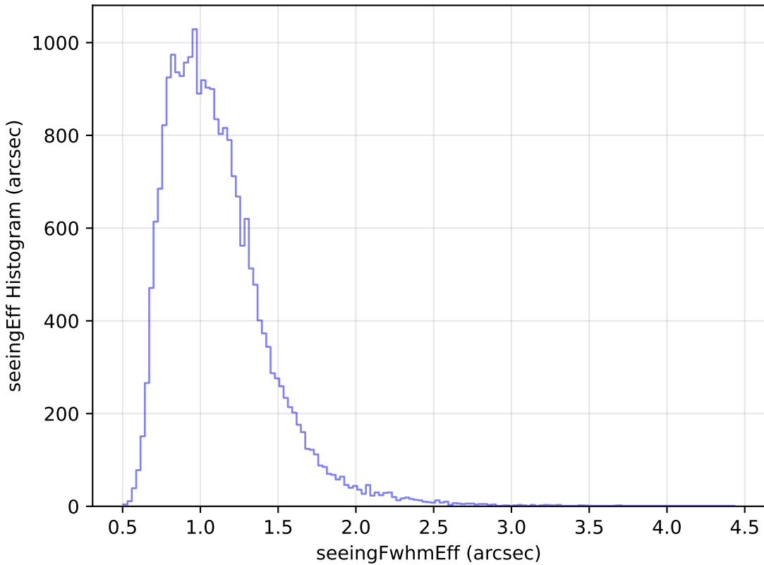
too_elab_r8_d3_gz_v3.4_10yrs Yr 1 g band: seeingEff Histogram
