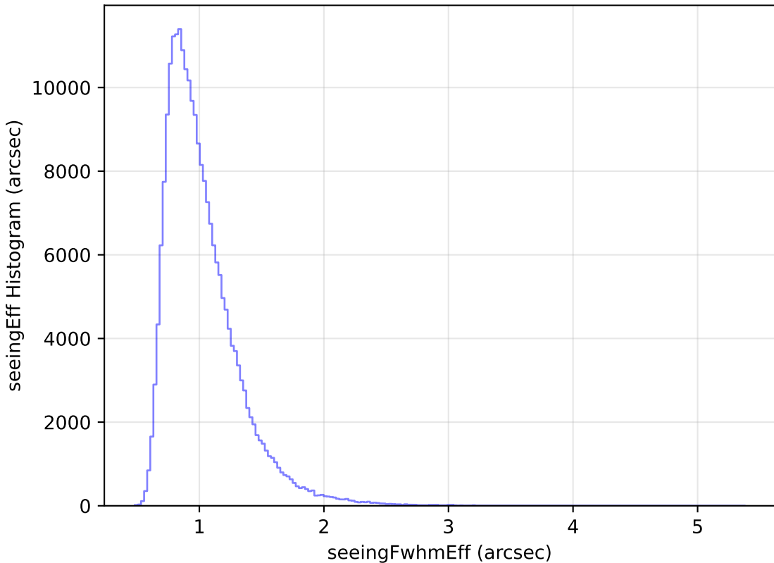
too_elab_r8_d3_gz_v3.4_10yrs Yr 1 all bands: seeingEff Histogram
