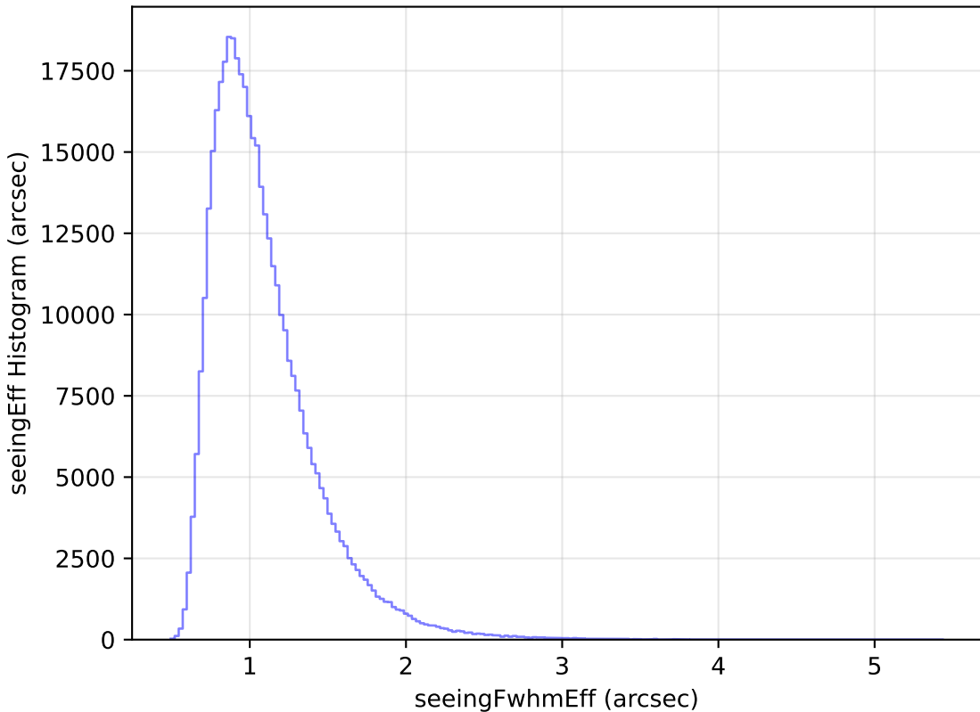
too_elab_r8_d3_gz_v3.4_10yrs WFD z band: seeingEff Histogram
