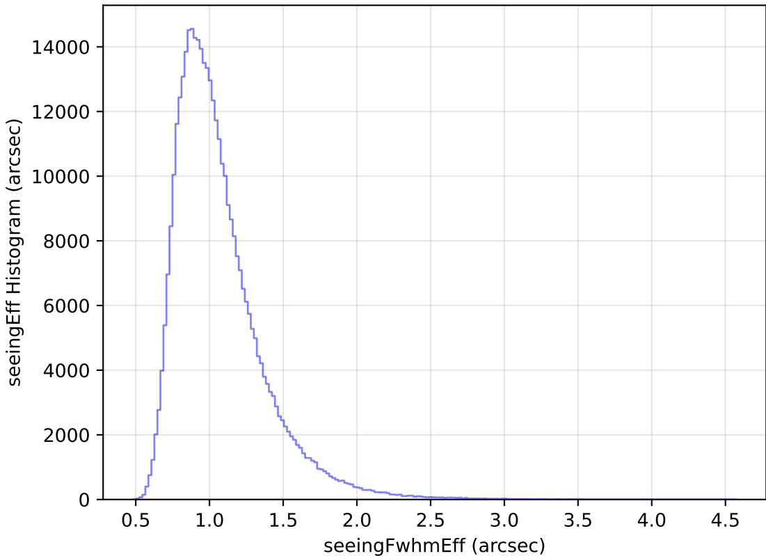
too_elab_r8_d3_gz_v3.4_10yrs WFD y band: seeingEff Histogram
