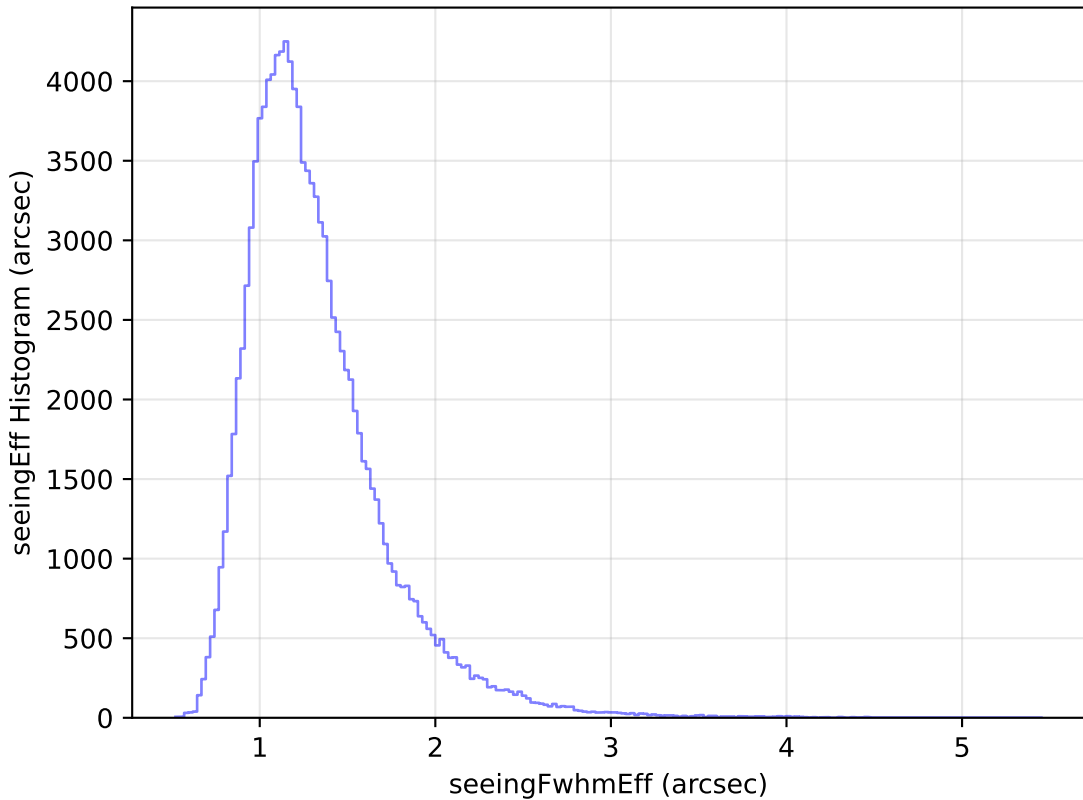
too_elab_r8_d3_gz_v3.4_10yrs WFD u band: seeingEff Histogram
